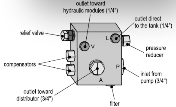
BCP02 - Max oil flow 140 lt/min
