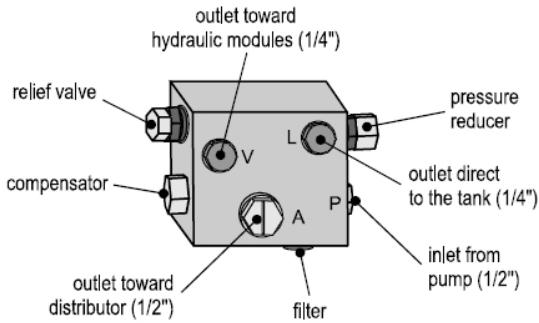
BCP01 - Max oil flow 70 lt/min
